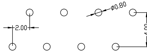
TYPE B PCB LAYOUT
