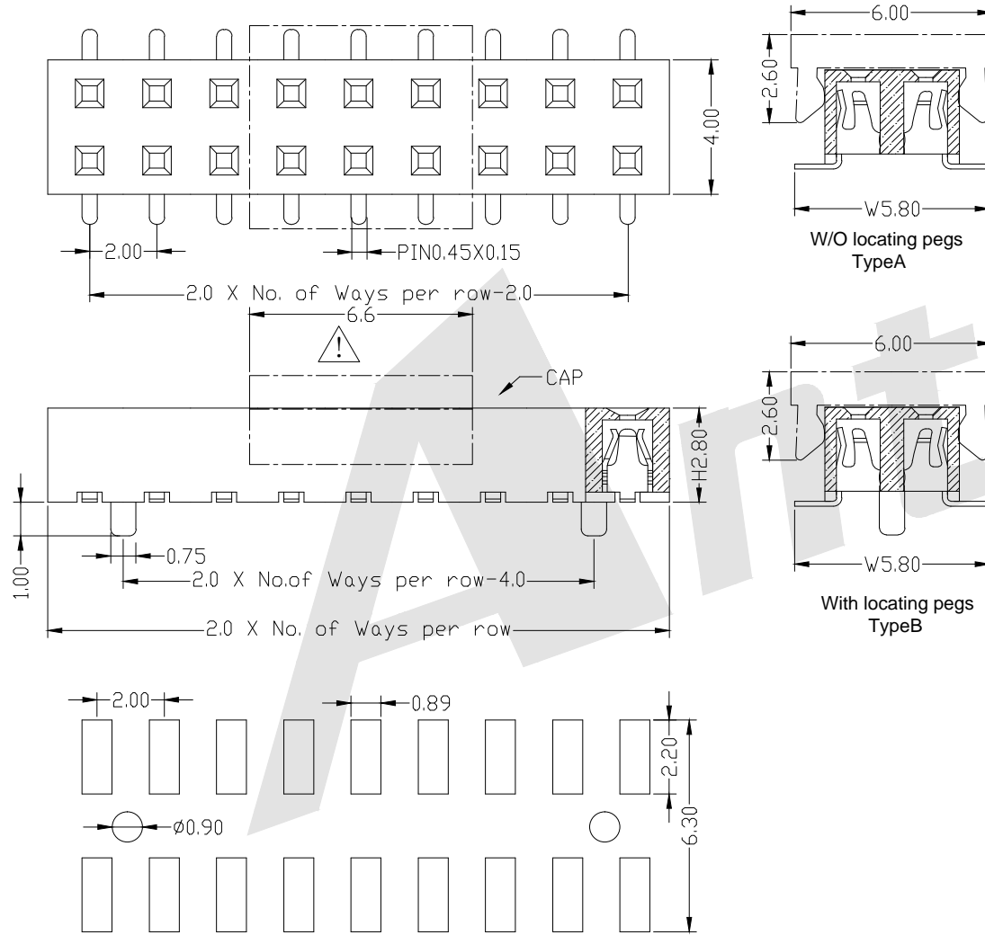
PCB LAYOUT
