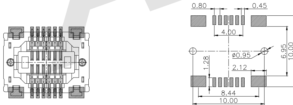
Recommended P.C.Board Layout (Tolerance:±0.05)
